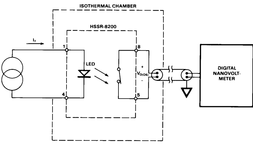
Figure 18. Voltage Offset Test Setup.
