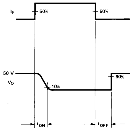
Figure 10. Switching Test Circuit for t_{ON} , t_{OFF} .
